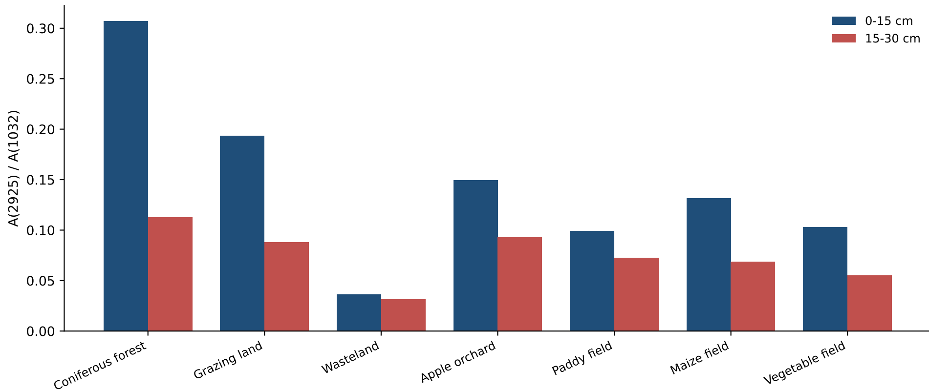
Aliphatic C-H to silicate band ratio - organic enrichment by land use and depth (simulated)
