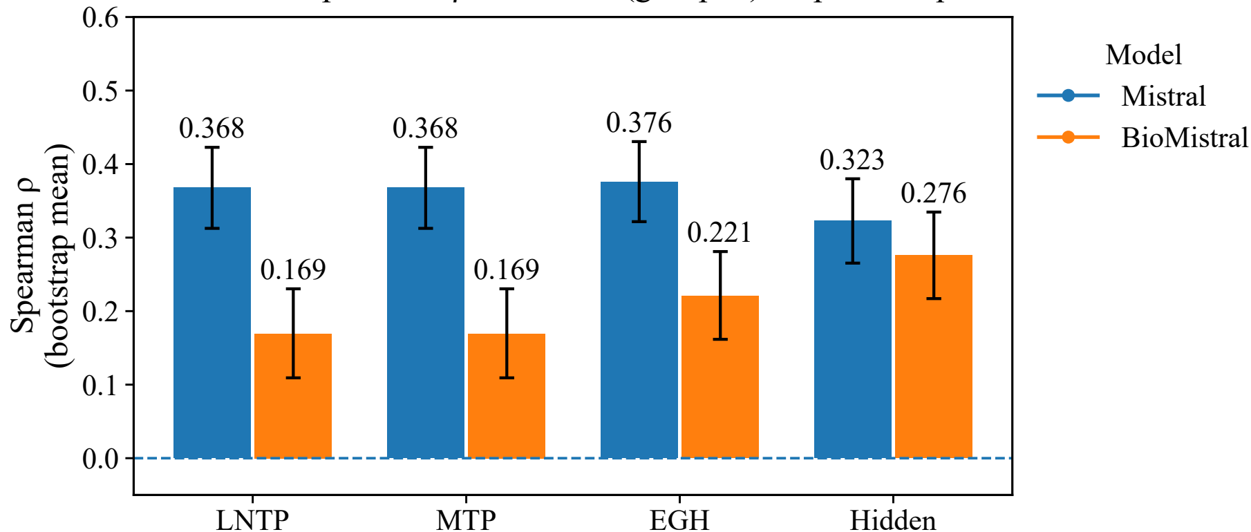
Phase 2 Spearman \rho + 95% CI (grouped) — pubmedqa
