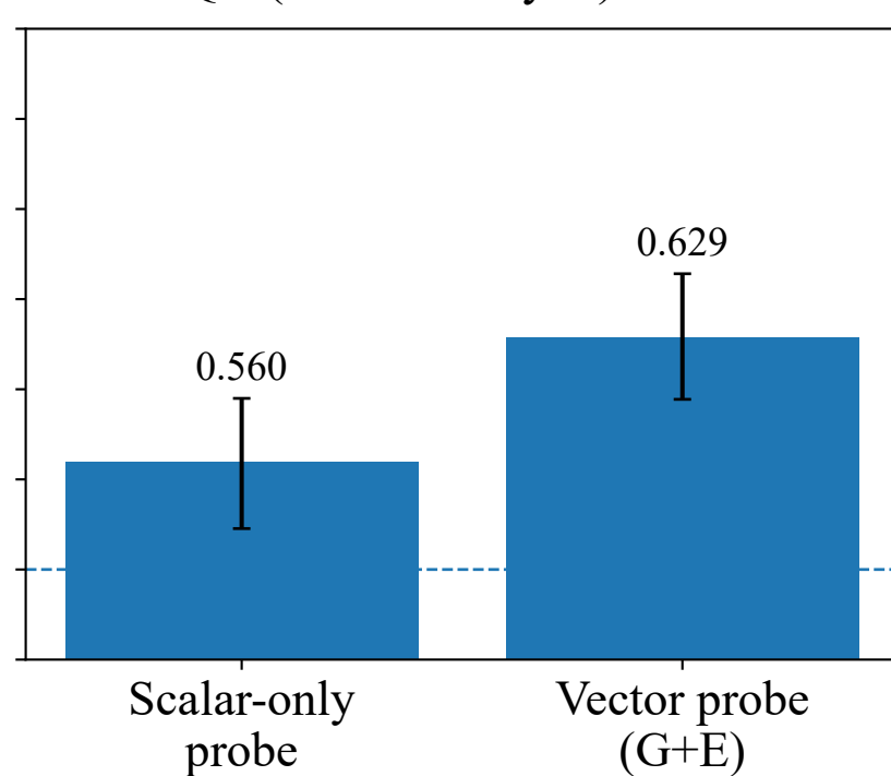
PubMedQA (Yes/No/Maybe) — BioMistral
