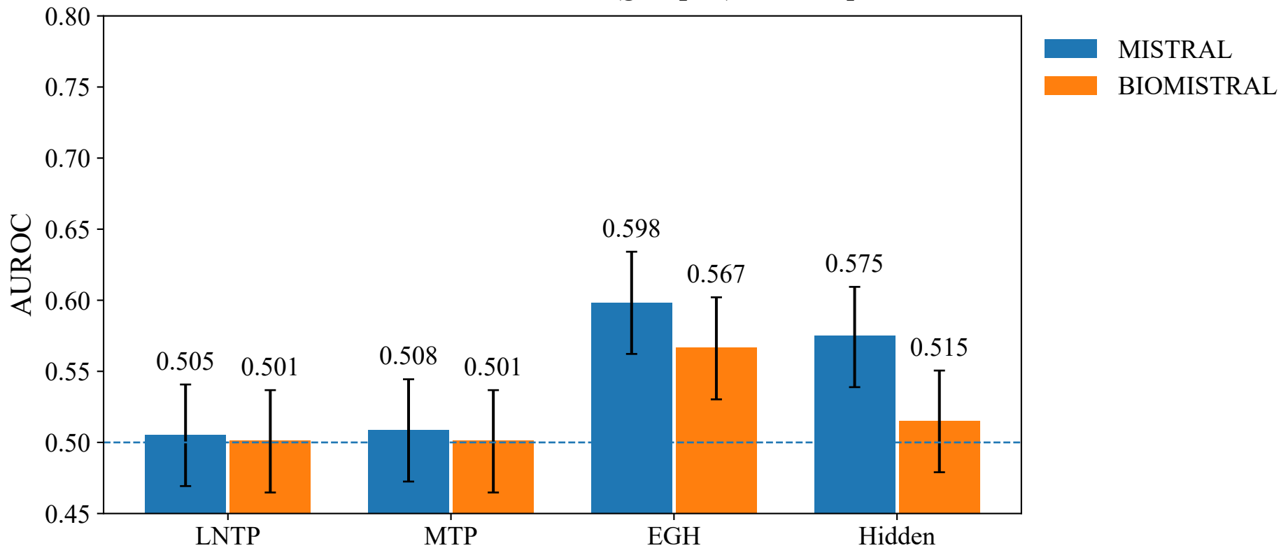
Phase 2 AUROC + 95% CI (grouped) — medqa
