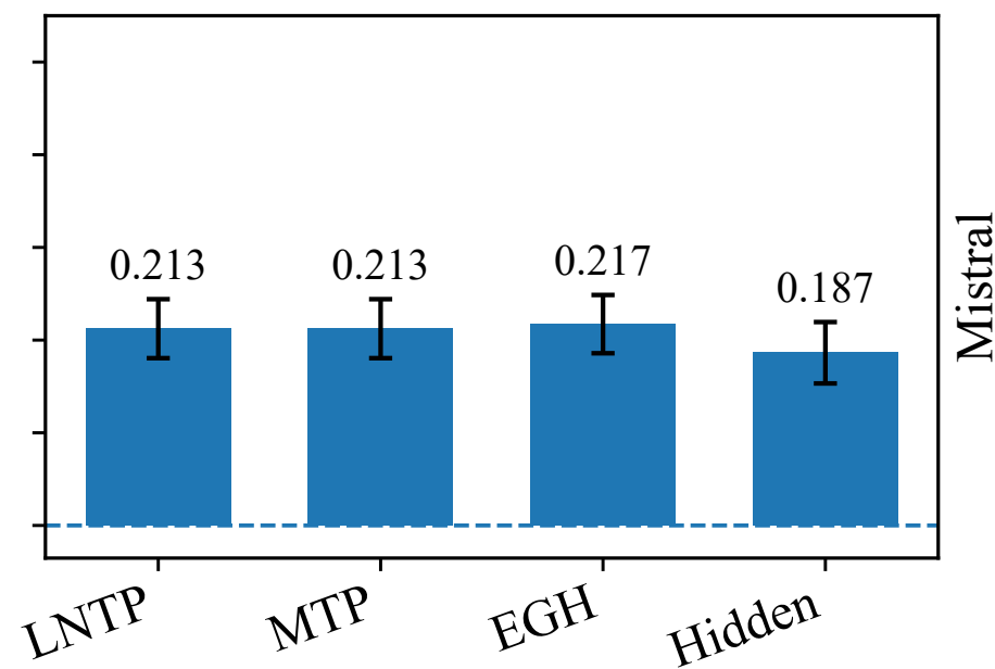
PubMedQA (Ternary)
