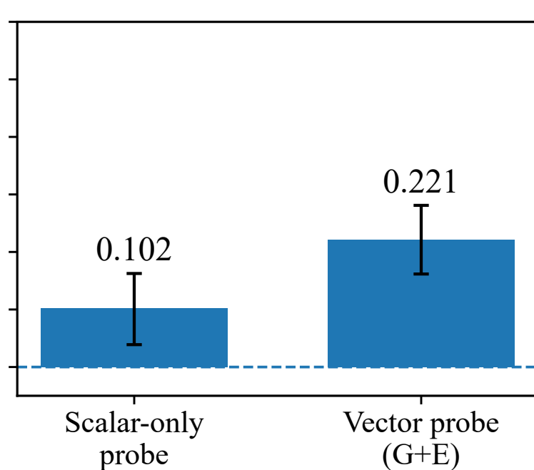
PubMedQA (Ternary) — BioMistral
