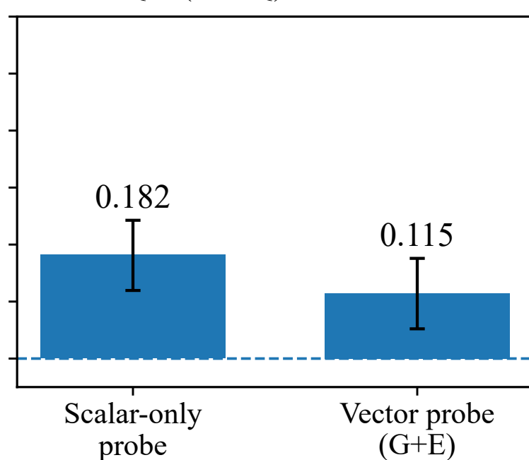
MedQA (MCQ) — BioMistral
