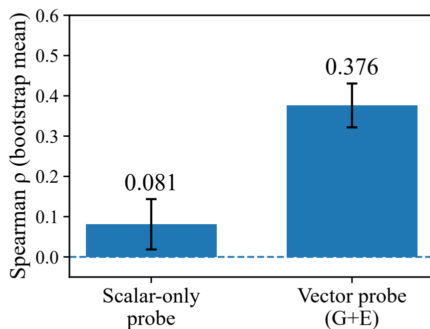
PubMedQA (Ternary) — Mistral
