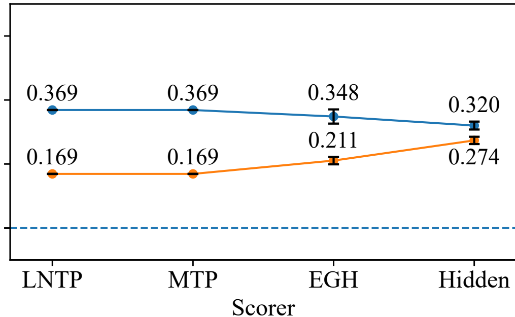
PubMedQA (Ternary)
