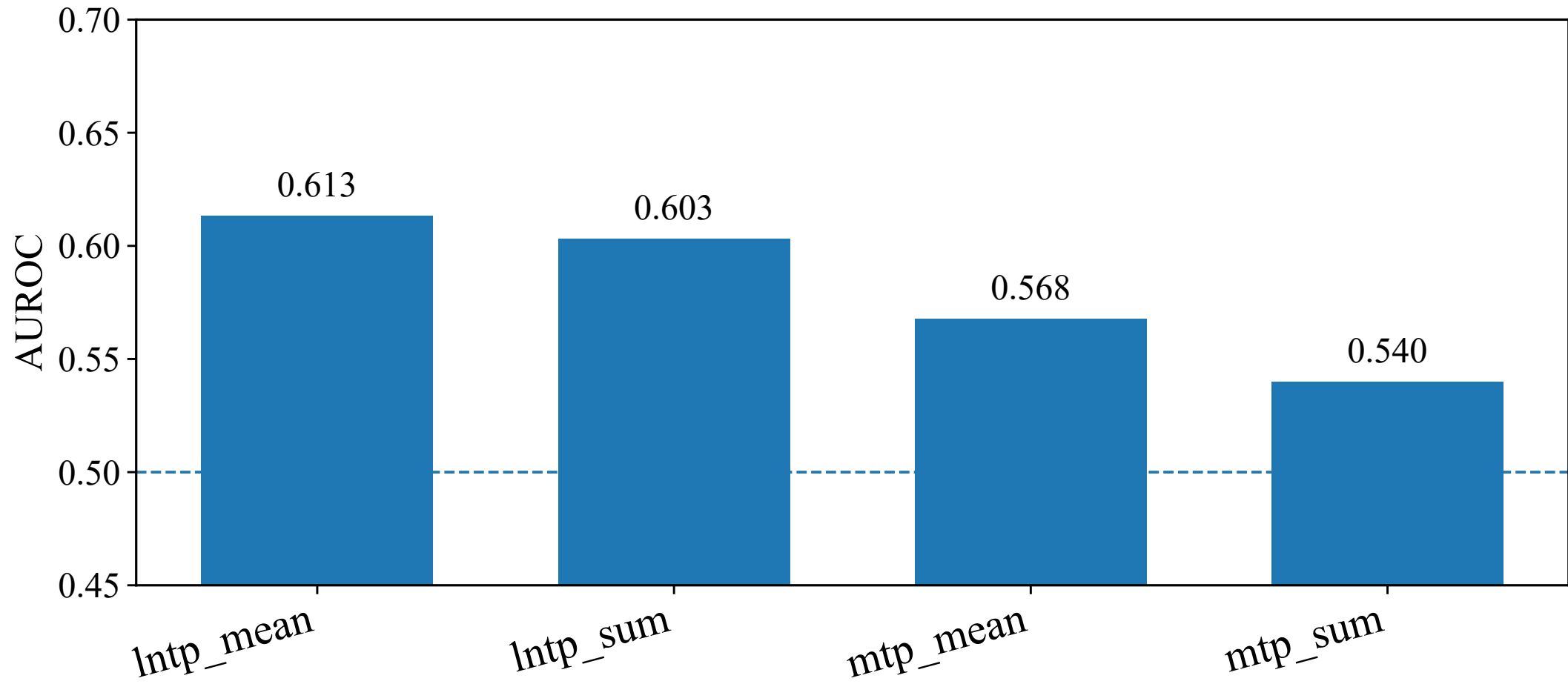
Token Score Bias — Length Normalization (AUROC) — mistral
