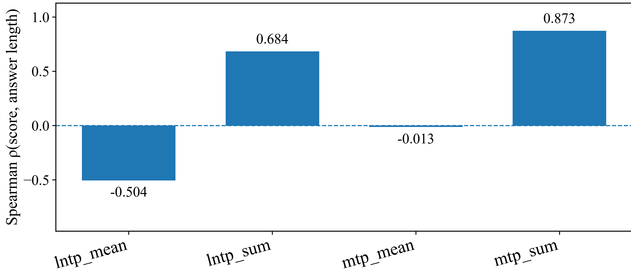
Token Score Bias — Length Dependence (Spearman) — mistral
