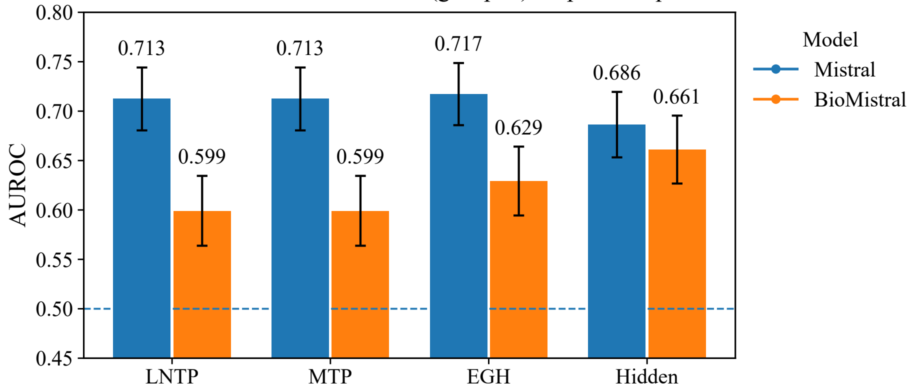
Phase 2 AUROC + 95% CI (grouped) — pubmedqa
