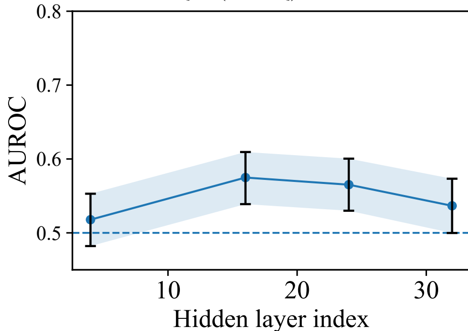
MedQA (MCQ) — Mistral
