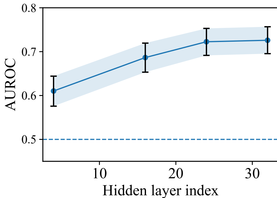
PubMedQA (Yes/No/Maybe) — Mistral
