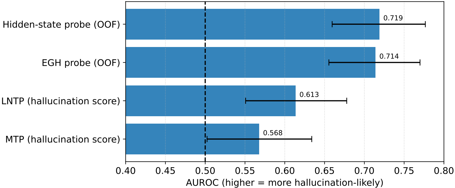
Figure 1 — AUROC Comparison (TruthfulQA, Frozen Answers)
