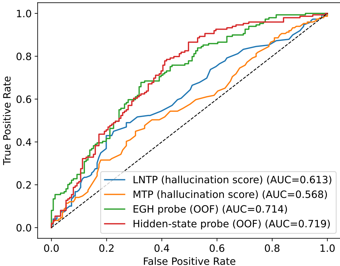
ROC Curves — Phase 1 (TruthfulQA)
