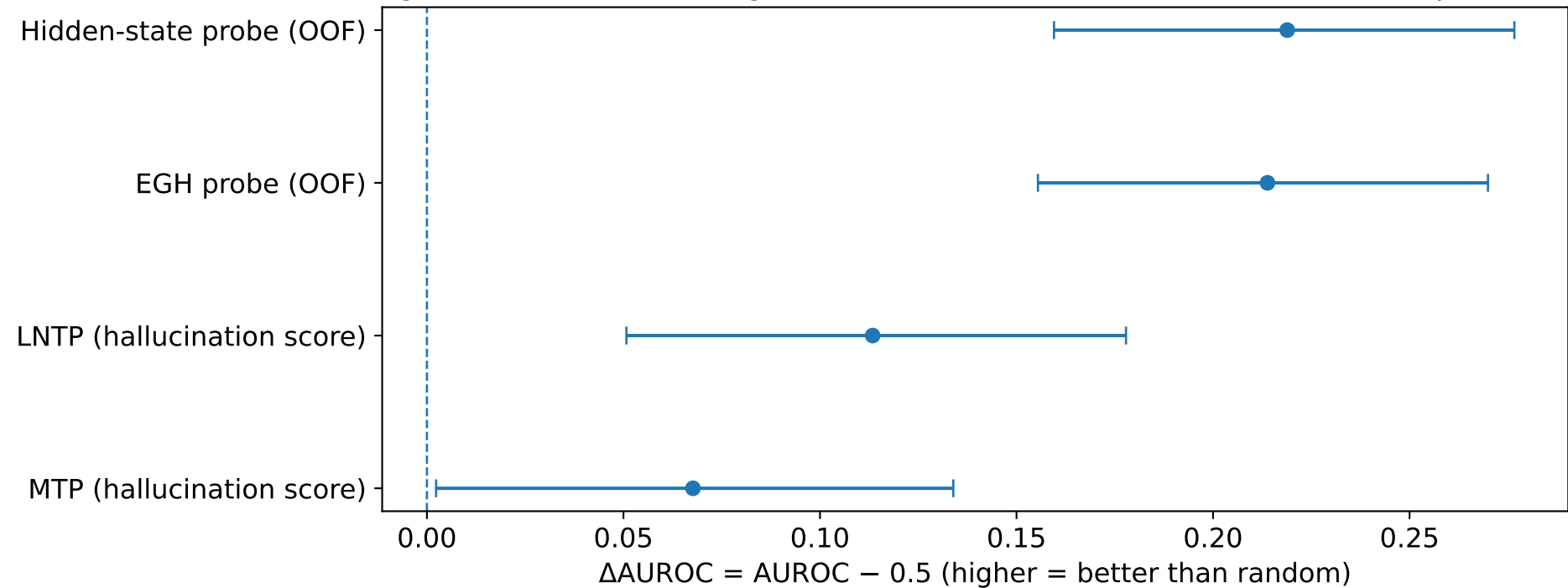
Figure B — AUROC margin above random ( \Delta\text{AUROC} ) with bootstrap 95% CI
