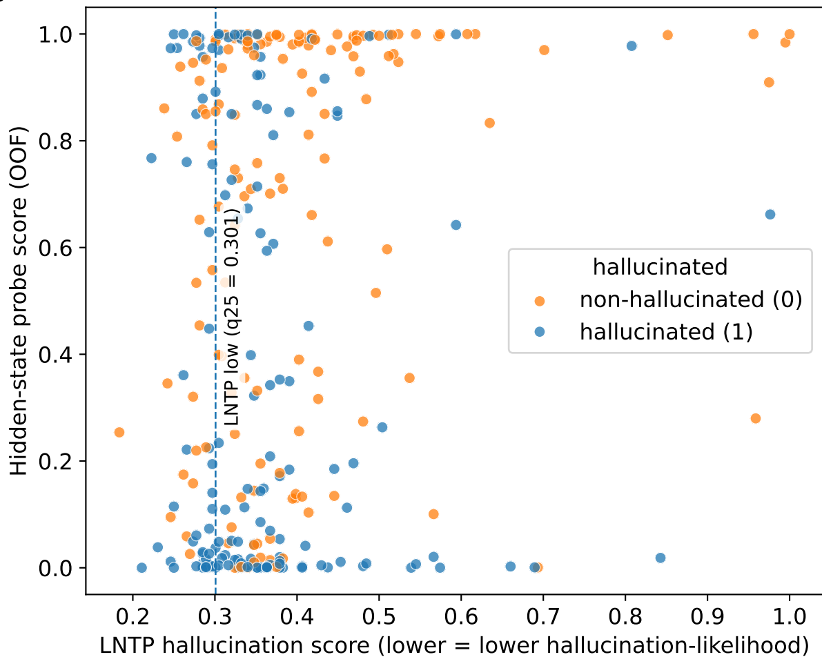
Figure E — LNTP-low mismatches (low LNTP score vs Hidden-state probe)
