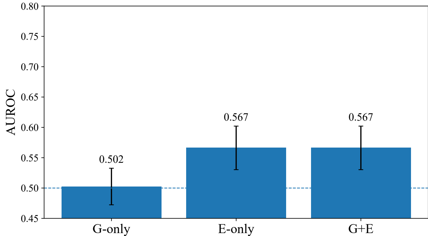
MedQA (MCQ) — BioMistral
