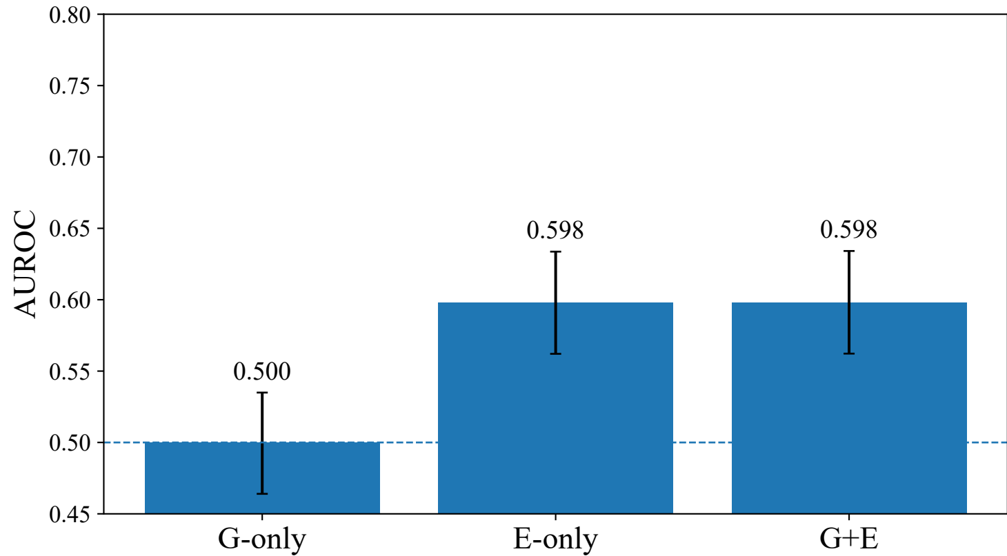
MedQA (MCQ) — Mistral
