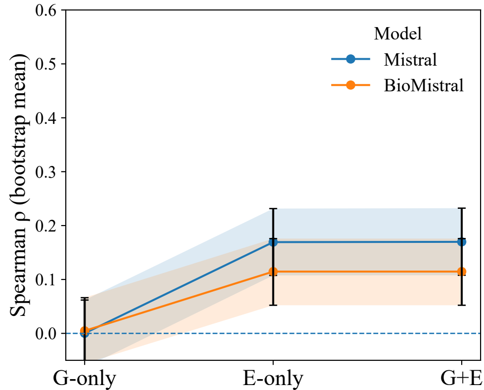
Ablation: EGH Probe Design (G-only vs E-only vs G+E) — Spearman \rho \pm 95\% CI MedQA (MCQ) PubMedQA (Yes/No/Maybe)
