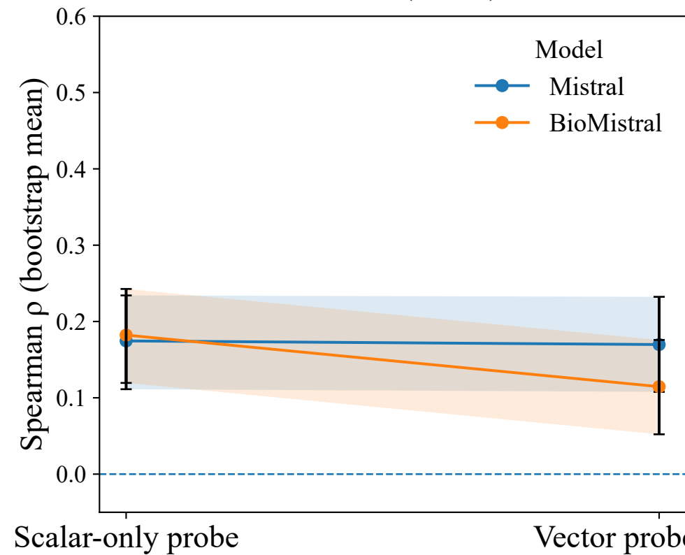
Ablation: EGH Scalar-only vs Vector Probe — Spearman \rho \pm 95\% CI MedQA (MCQ) PubMedQA (Yes/No/Maybe)
