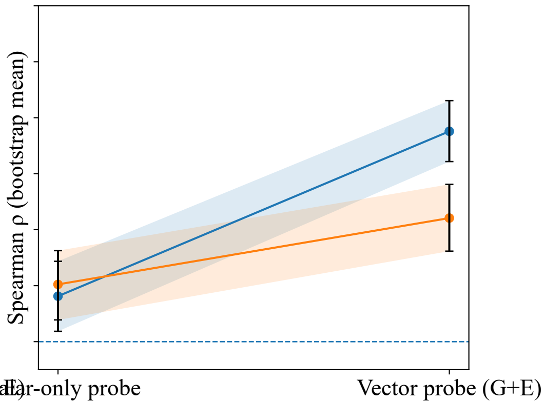
Ablation: EGH Scalar-only vs Vector Probe — Spearman \rho \pm 95\% CI MedQA (MCQ) PubMedQA (Yes/No/Maybe)
