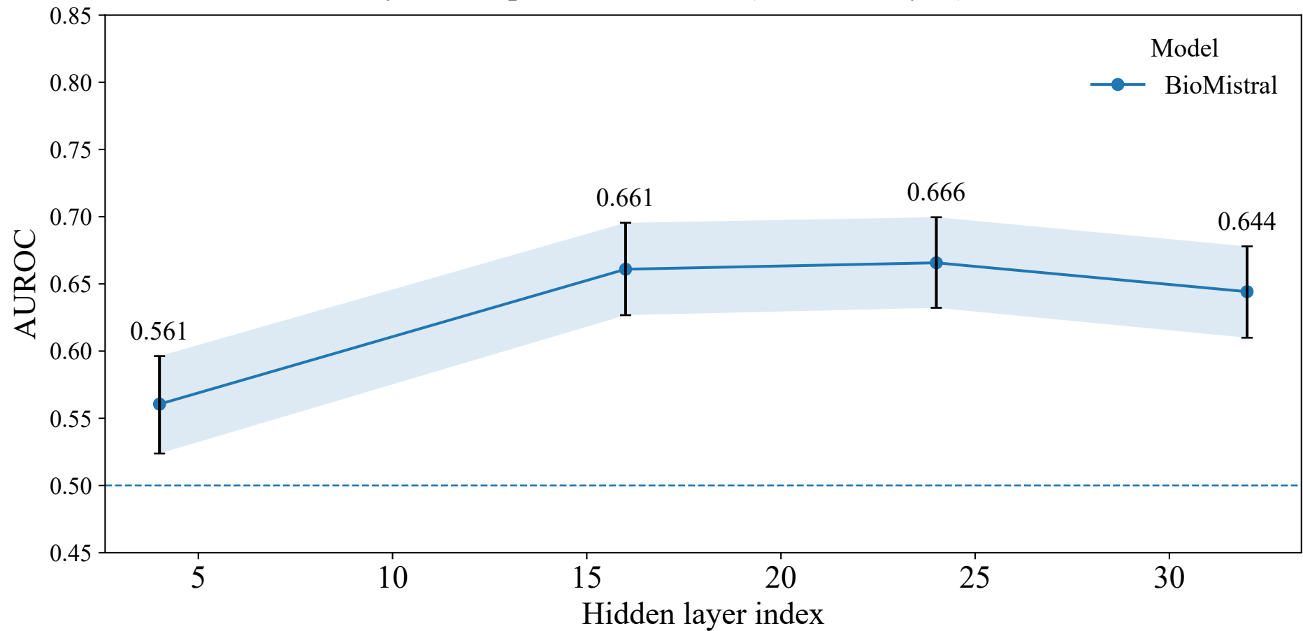
Hidden Layer Sweep — PubMedQA (Yes/No/Maybe) — BioMistral
