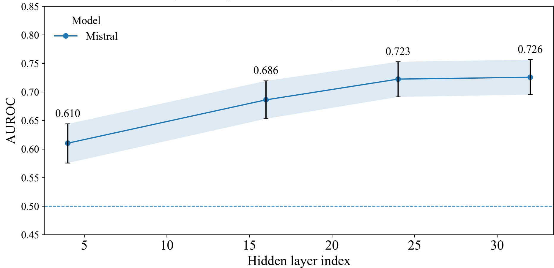
Hidden Layer Sweep — PubMedQA (Yes/No/Maybe) — Mistral
