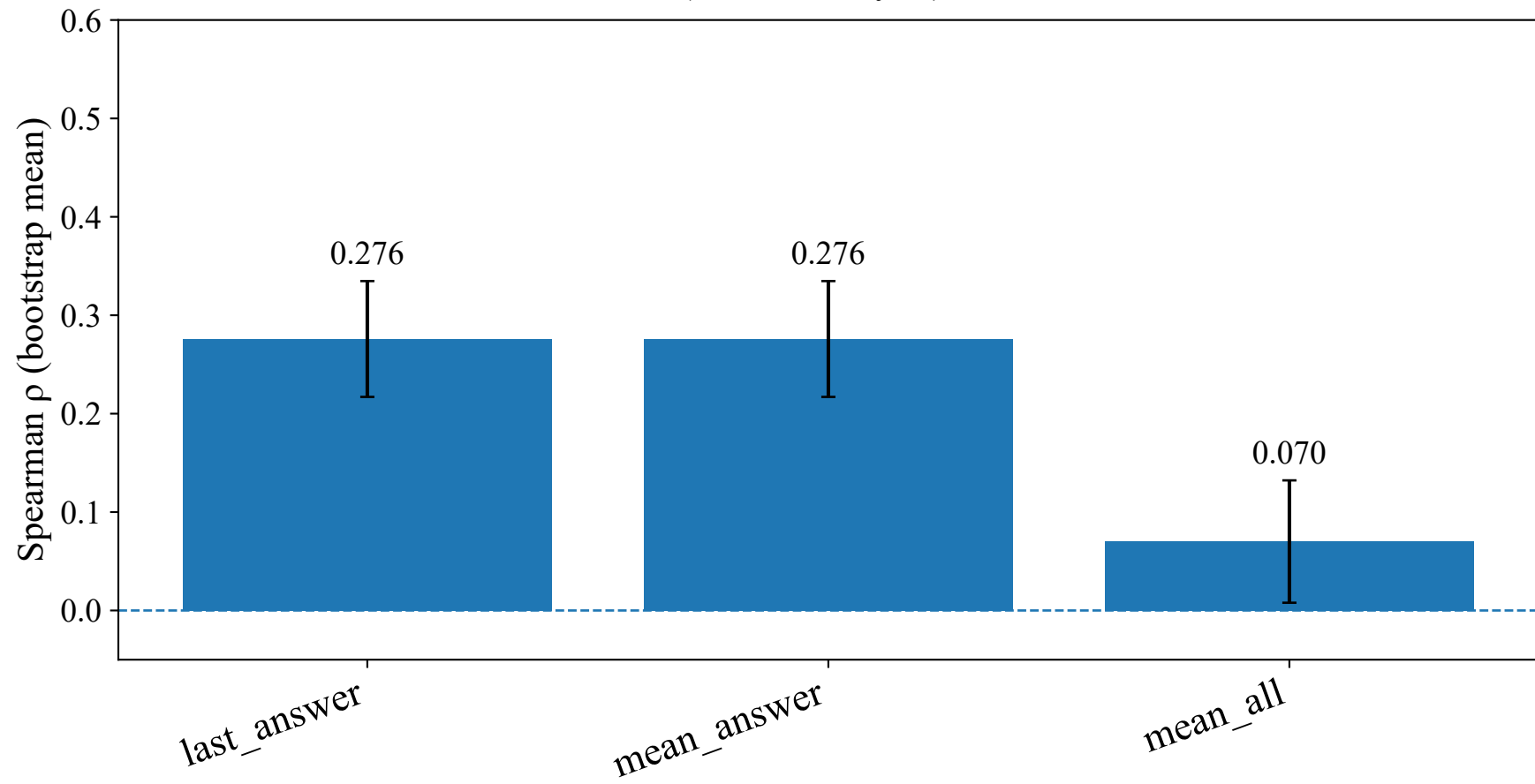
PubMedQA (Yes/No/Maybe) — BioMistral
