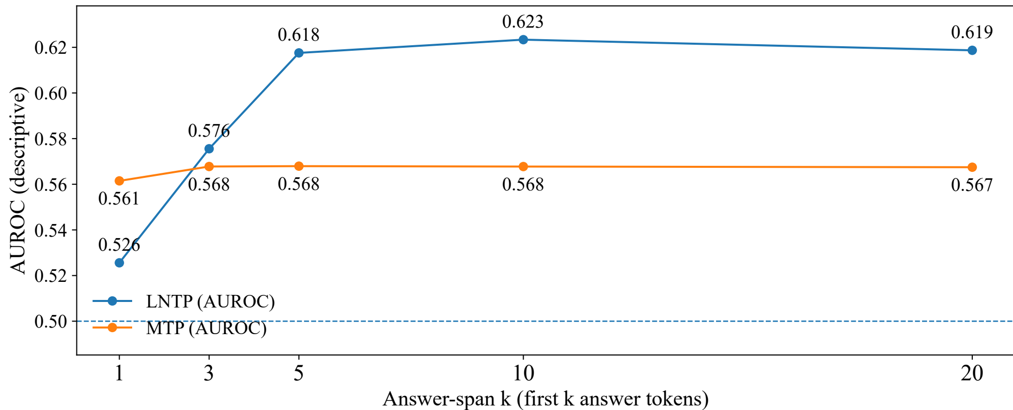
Token Score Bias — Answer-span k-sweep (AUROC vs k) — mistral
