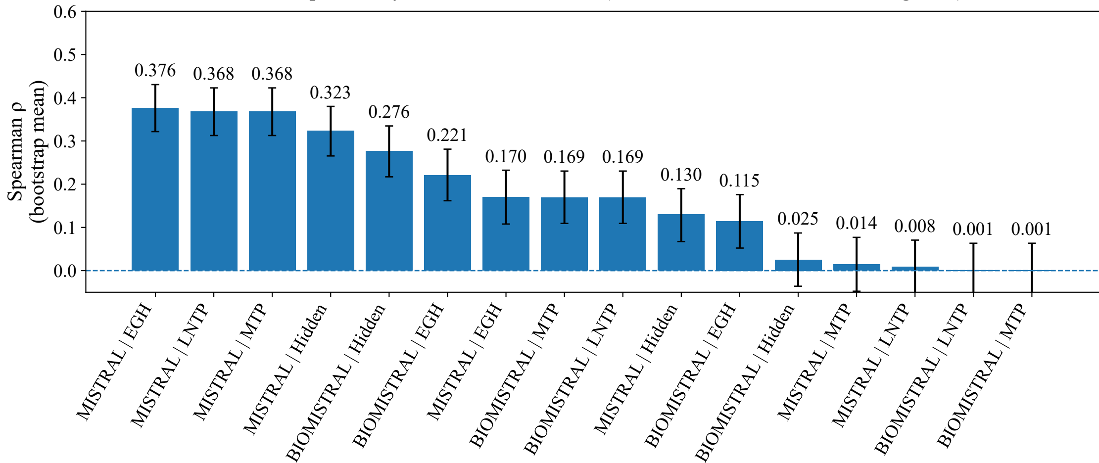
Phase 2 Spearman \rho + 95% CI — all runs (MedQA + PubMedQA shown together)
