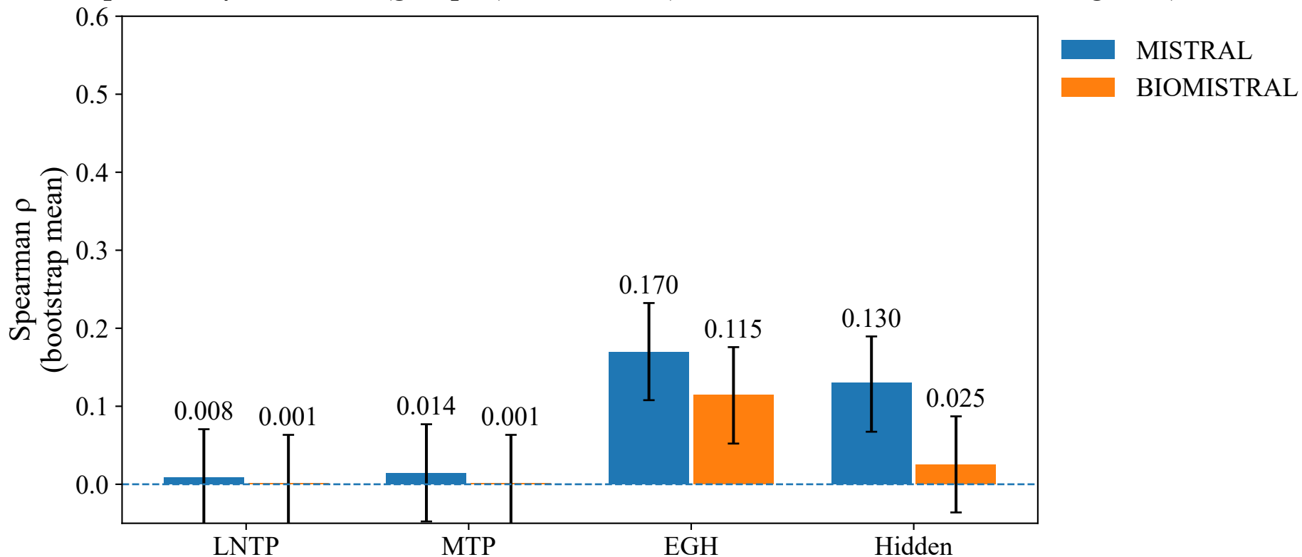
Phase 2 Spearman \rho + 95% CI (grouped) — all runs (MedQA + PubMedQA shown together)
