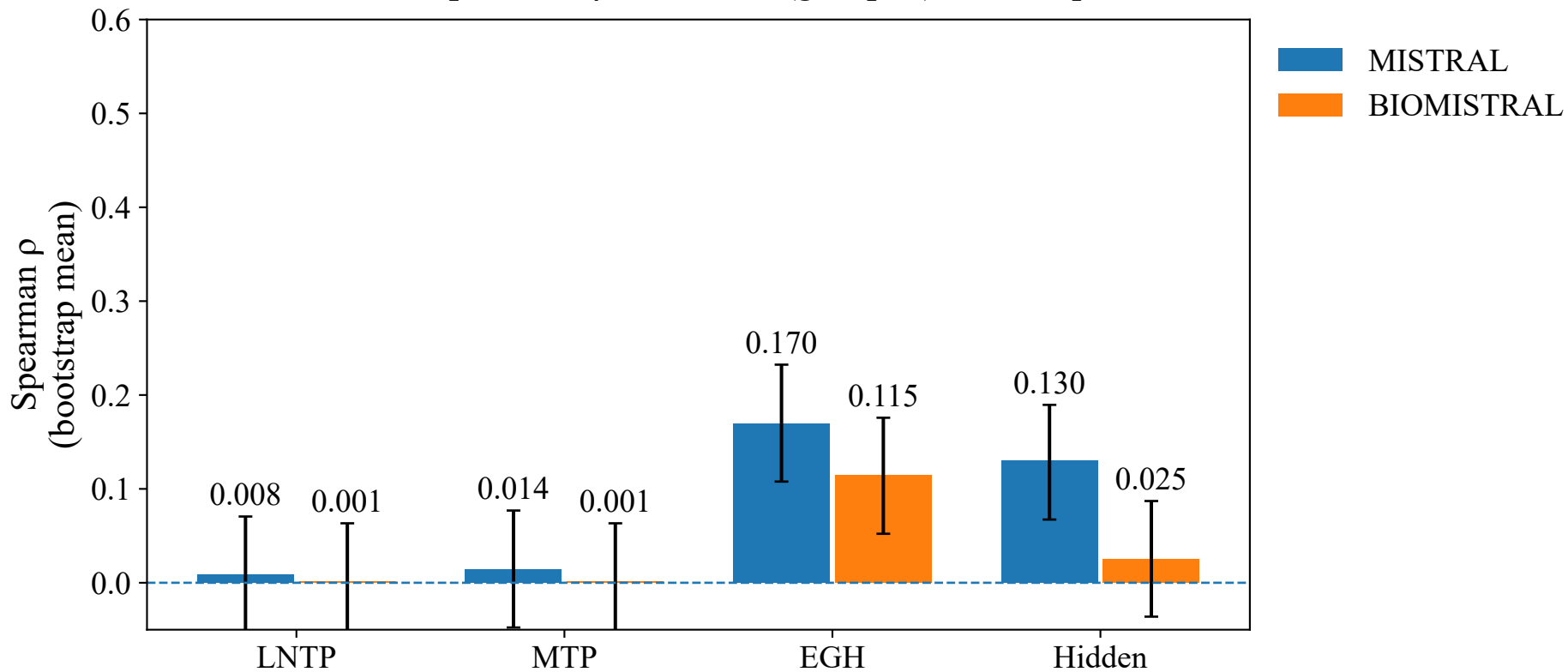
Phase 2 Spearman \rho + 95% CI (grouped) — medqa
