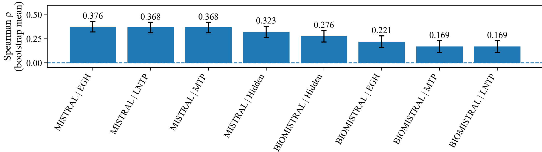
Phase 2 Spearman \rho + 95% CI — pubmedqa
