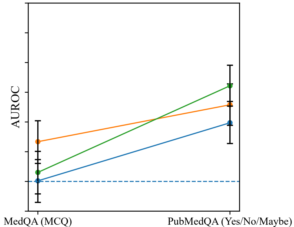
BioMistral
