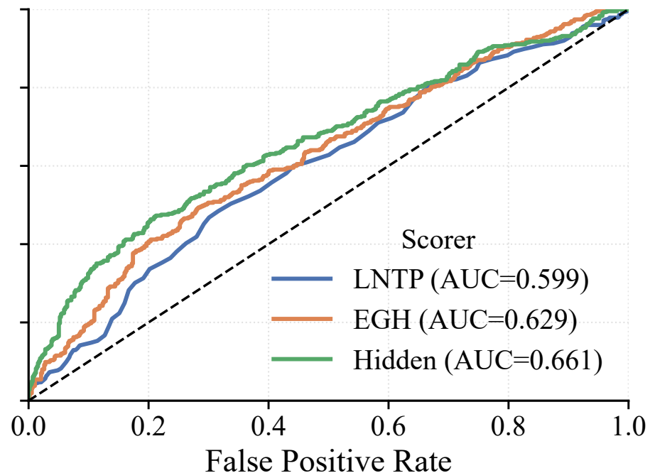
BioMistral
