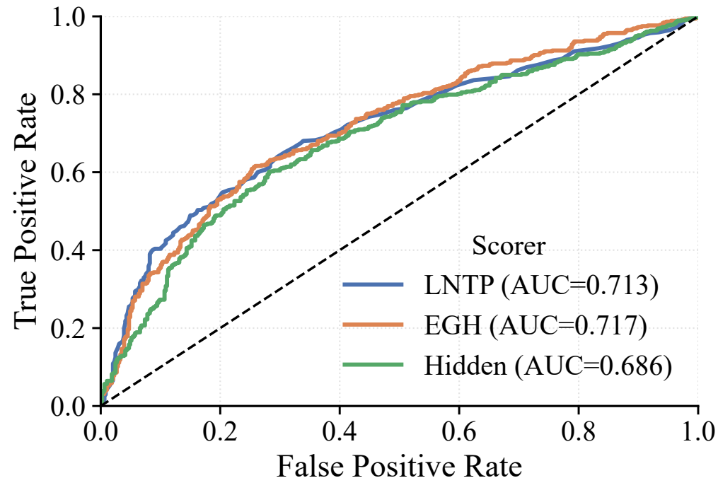
Mistral
