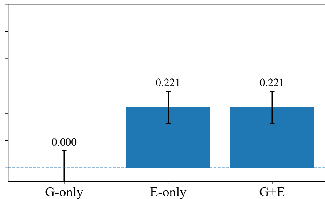
PubMedQA (Yes/No/Maybe) — BioMistral
