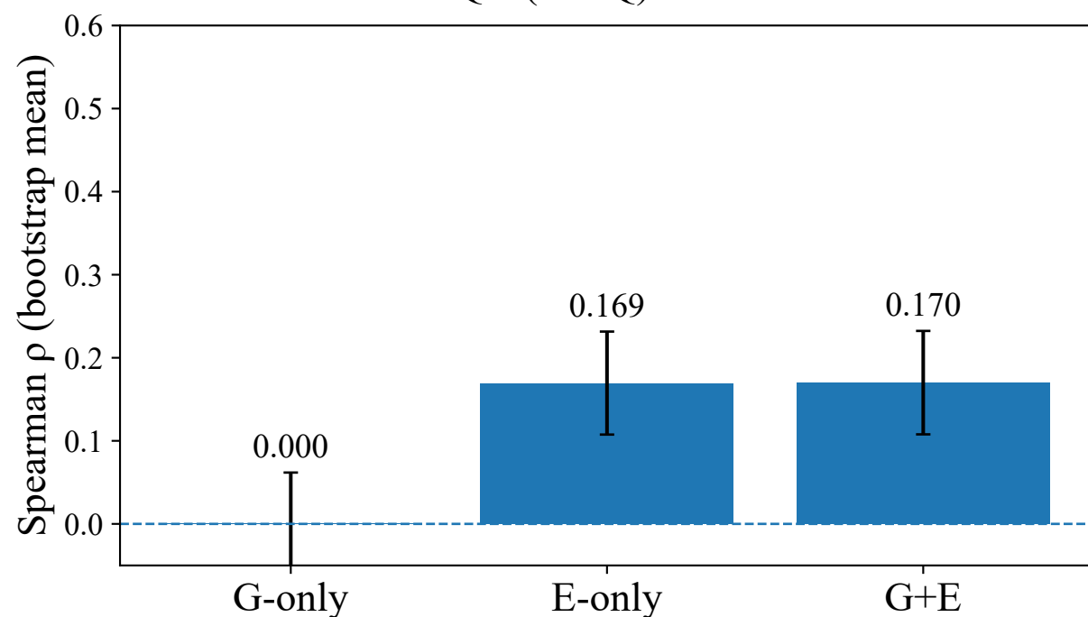
MedQA (MCQ) — Mistral
