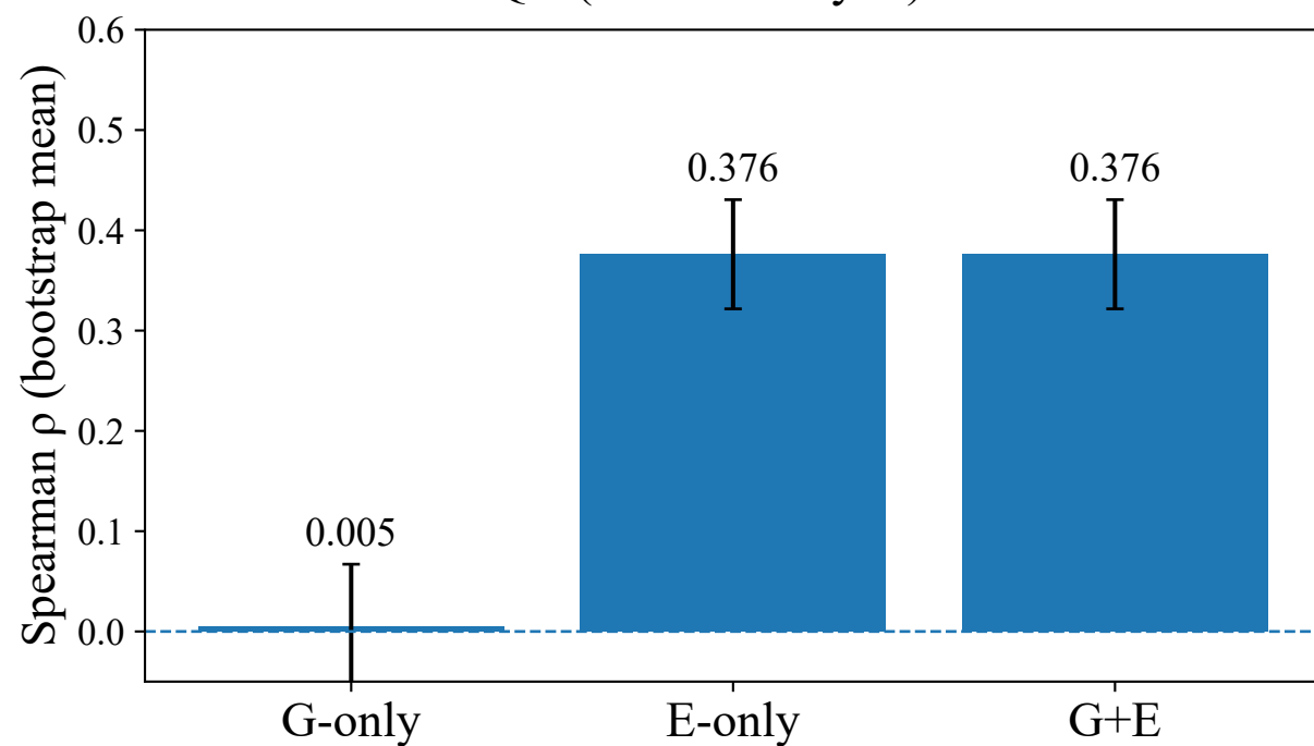
PubMedQA (Yes/No/Maybe) — Mistral
