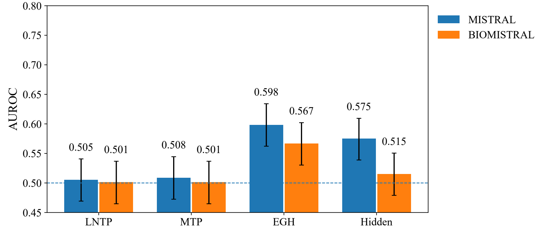
Phase 2 AUROC + 95% CI (grouped) — all runs (MedQA + PubMedQA shown together)
