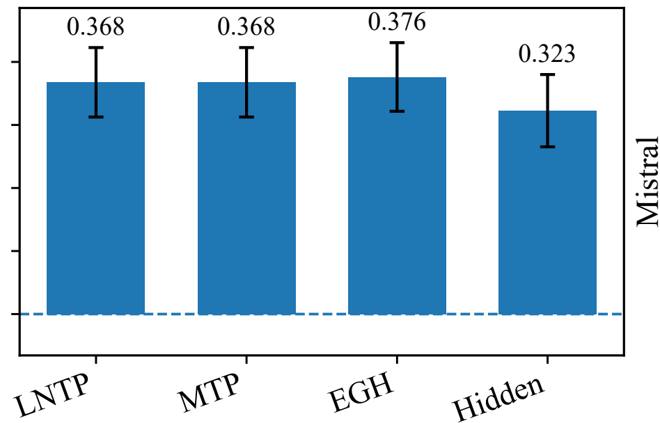
PubMedQA (Ternary)
