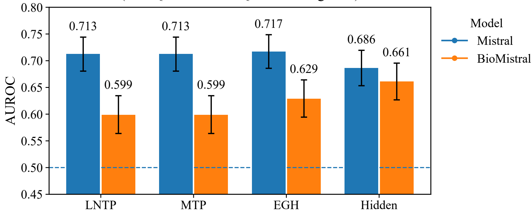
Phase 2 AUROC + 95% CI (grouped) — all runs (MedQA + PubMedQA shown together)
