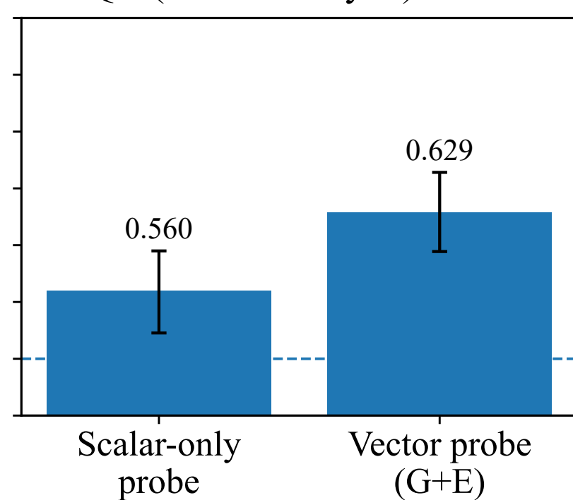
PubMedQA (Yes/No/Maybe) — Mistral
