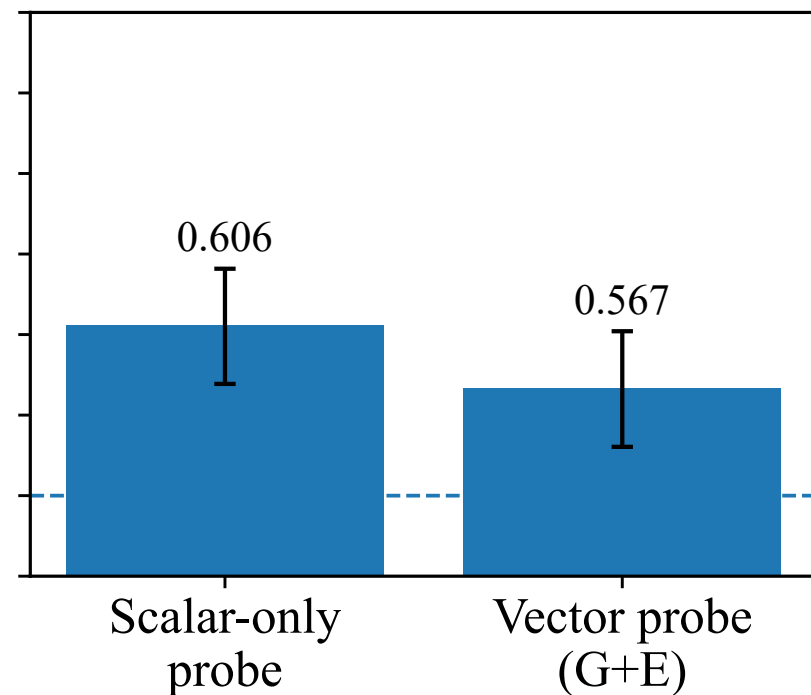
PubMedQA (Yes/No/Maybe) — Mistral
