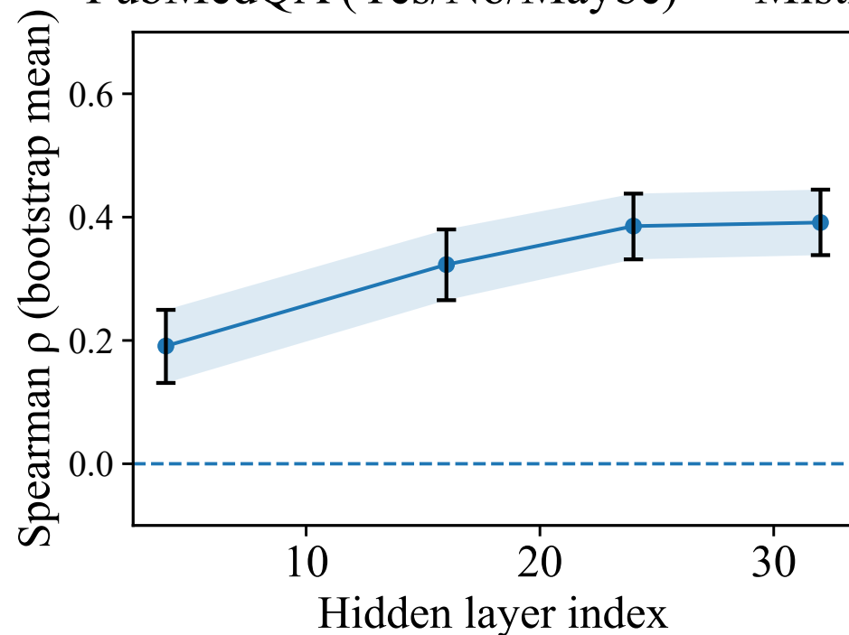
PubMedQA (Yes/No/Maybe) — Mistral
