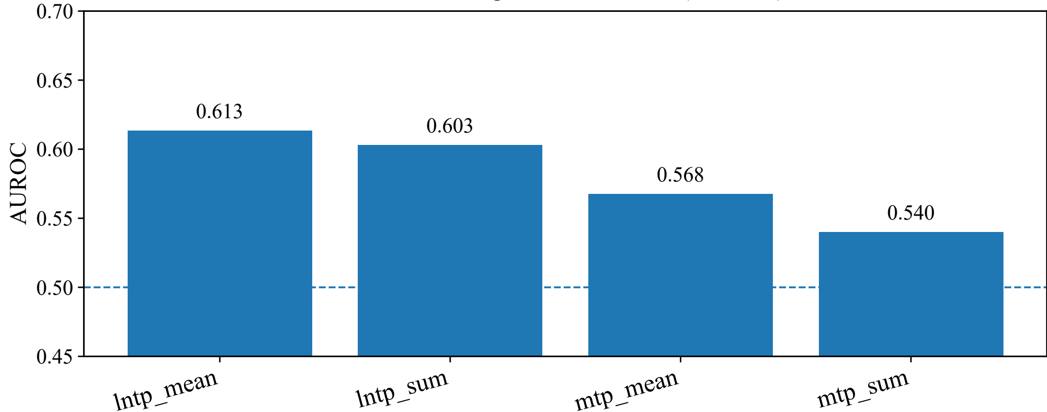
Token Score Bias — Length Normalization (AUROC) — mistral
