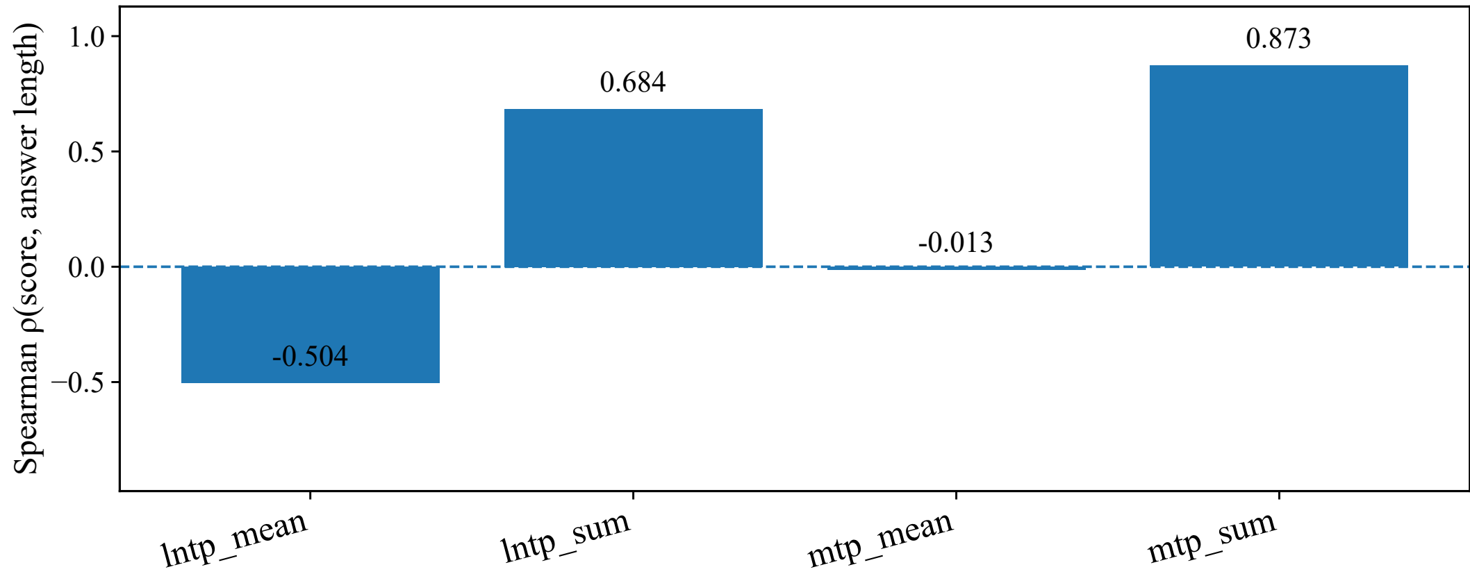
Token Score Bias — Length Dependence (Spearman) — mistral
