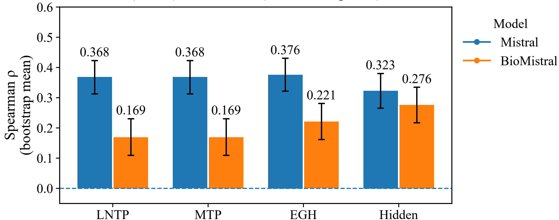
Phase 2 Spearman \rho + 95% CI (grouped) — all runs (MedQA + PubMedQA shown together)
