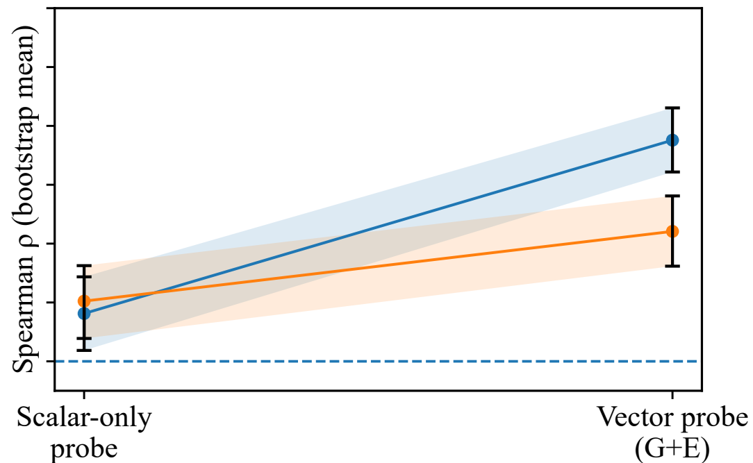
PubMedQA (Ternary)
