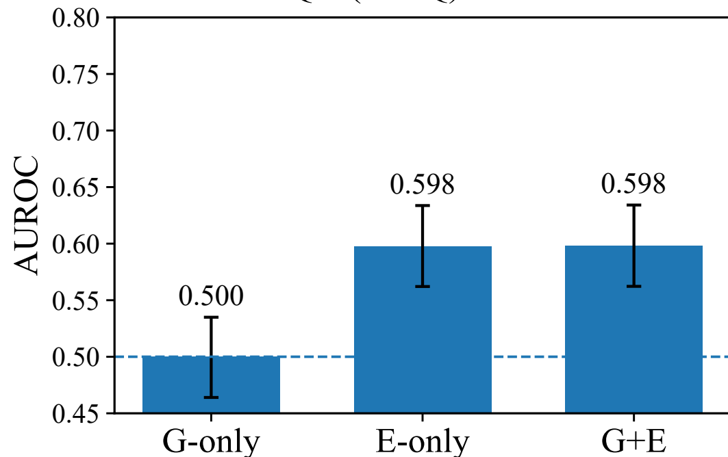
MedQA (MCQ) — Mistral
