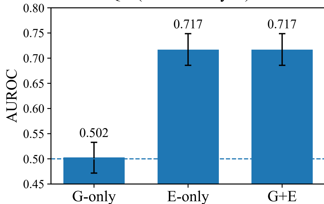
PubMedQA (Yes/No/Maybe) — Mistral
