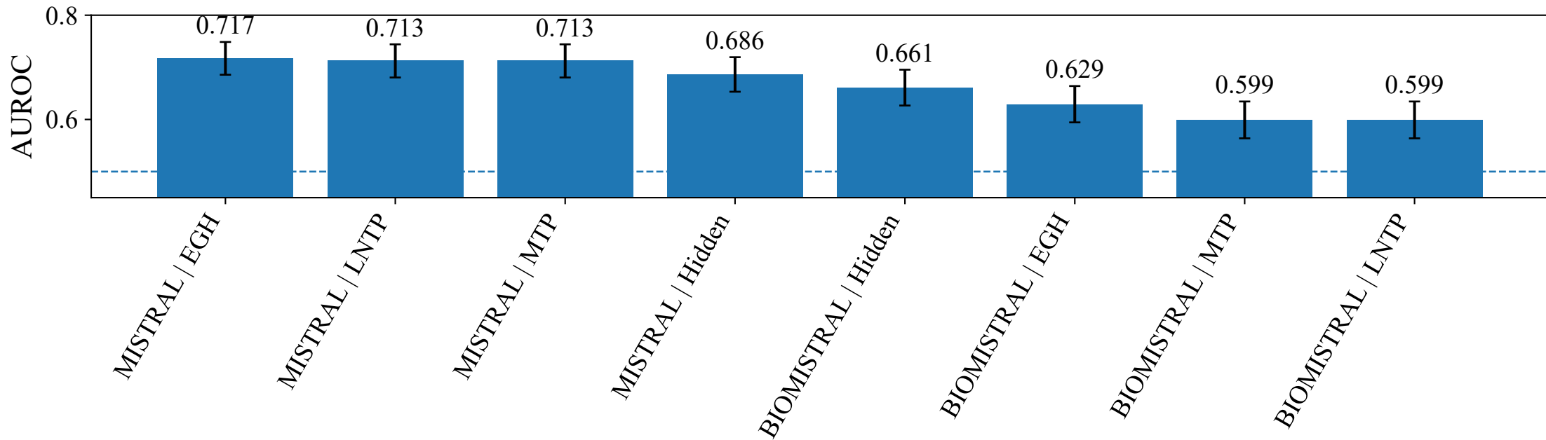
Phase 2 AUROC + 95% CI — pubmedqa
