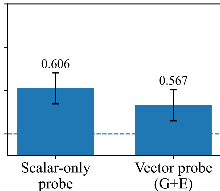
MedQA (MCQ) — BioMistral
