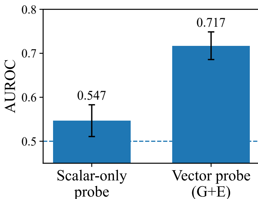
PubMedQA (Yes/No/Maybe) — Mistral
