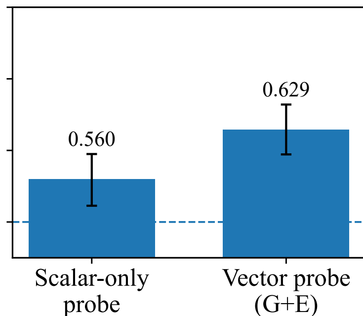
PubMedQA (Yes/No/Maybe) — BioMistral
