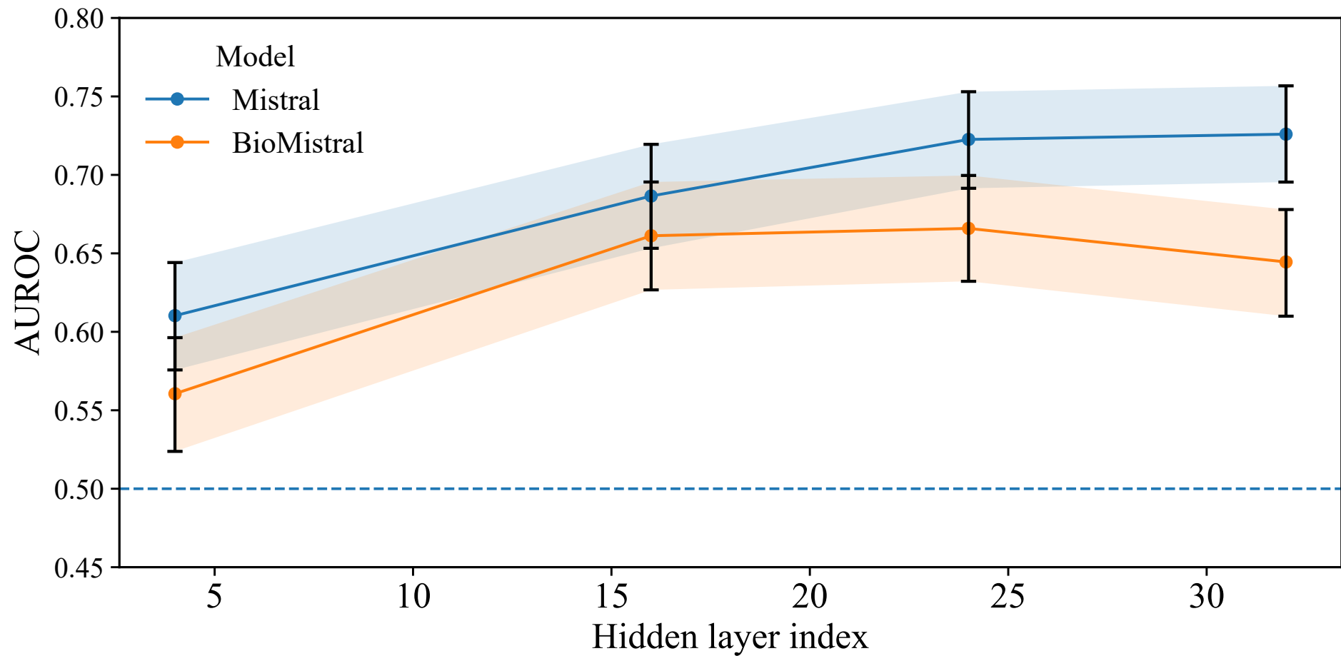
Hidden Layer Sweep — PubMedQA (Yes/No/Maybe) (Model overlay)
