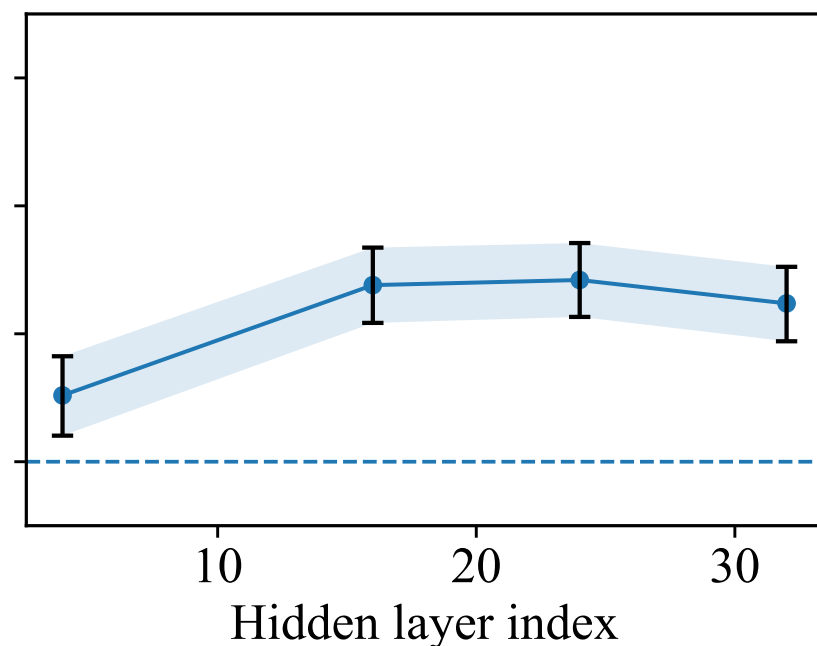
PubMedQA (Yes/No/Maybe) — BioMistral
