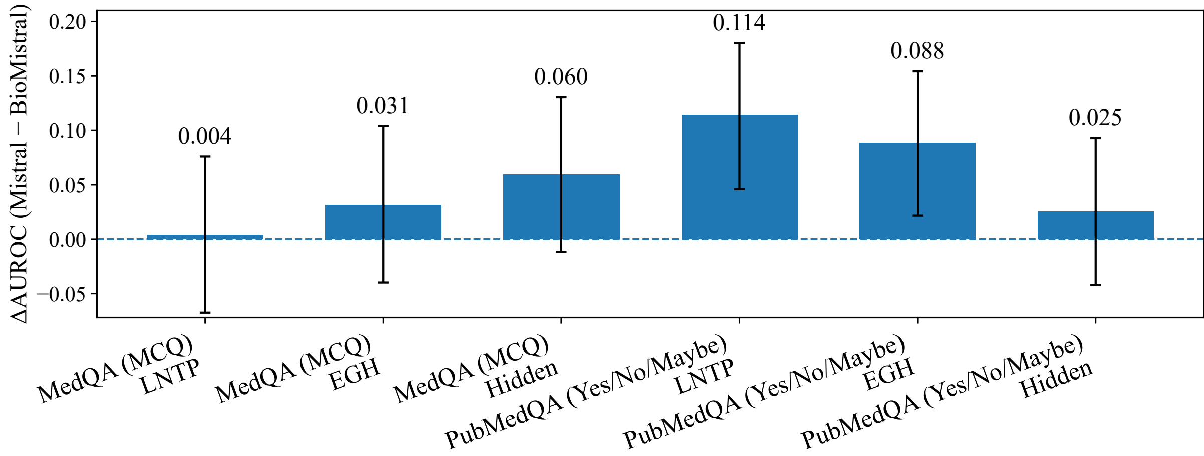
Model specialization effect (approx. CI via bounds)
