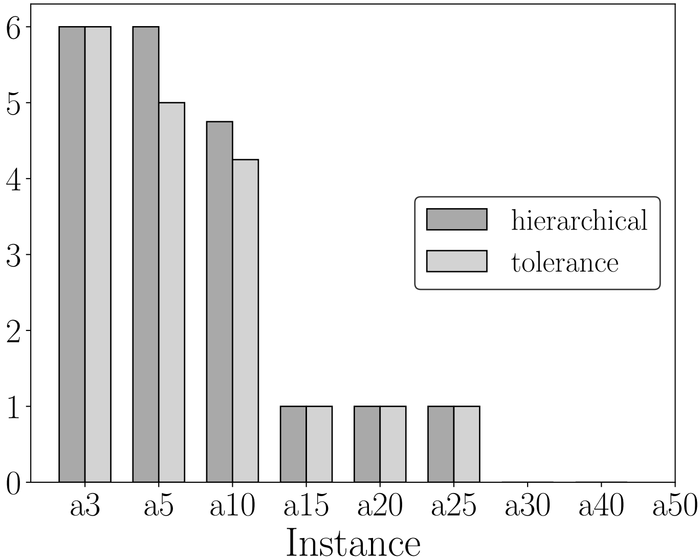
Achieved Objectives
