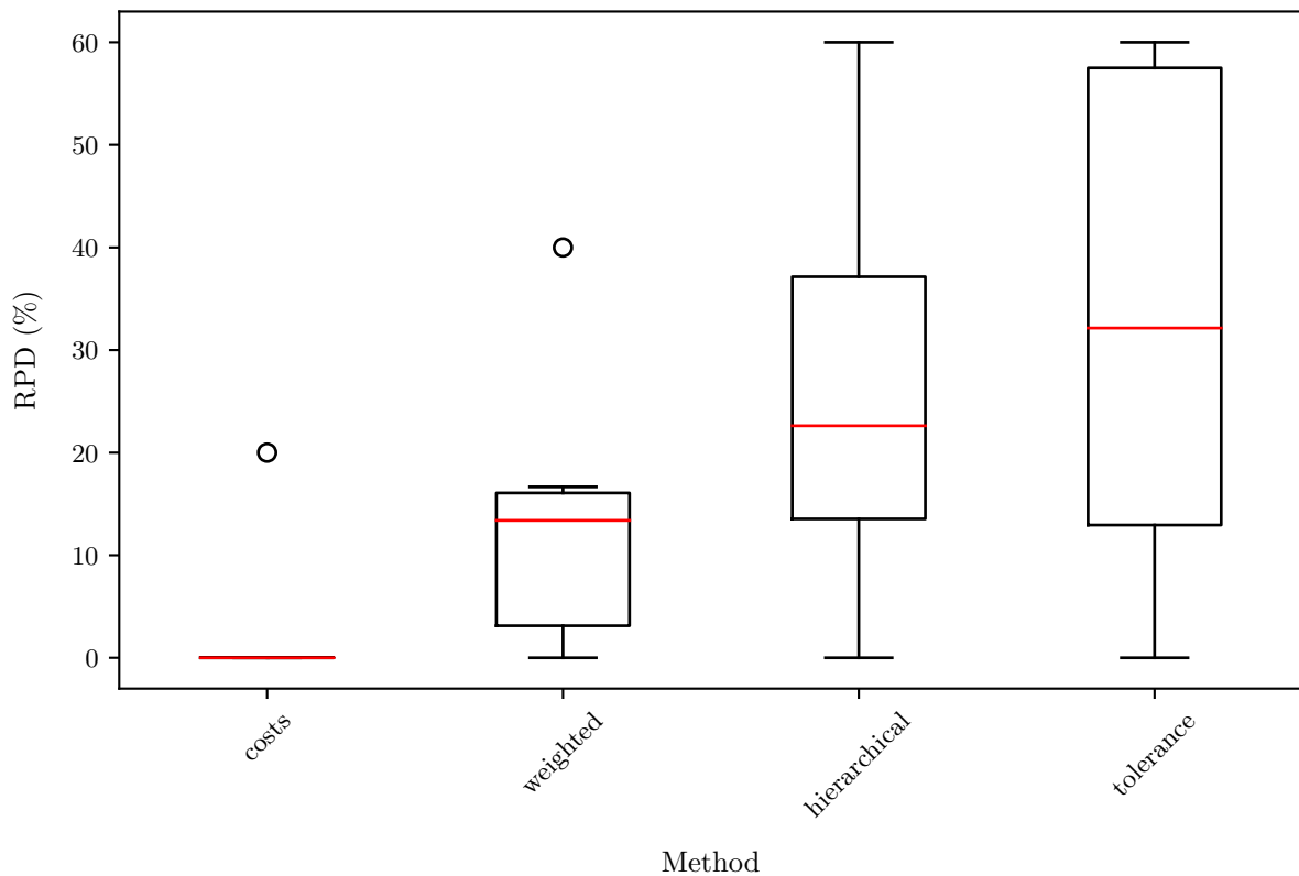
RPD Distribution for Worker Count
