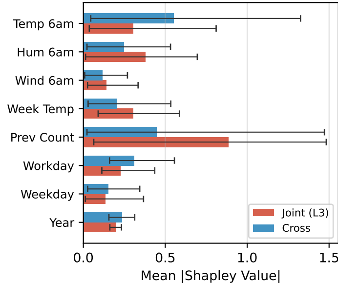
Global L3 vs Cross — |\phi| (mean, 5-95%)
