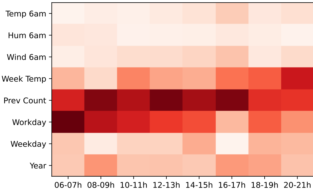
NGBoost Feature Importances for \mu (per horizon)
