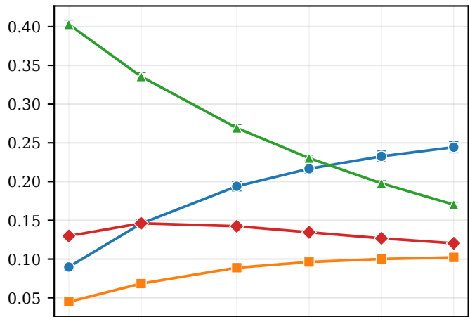
Student- t
